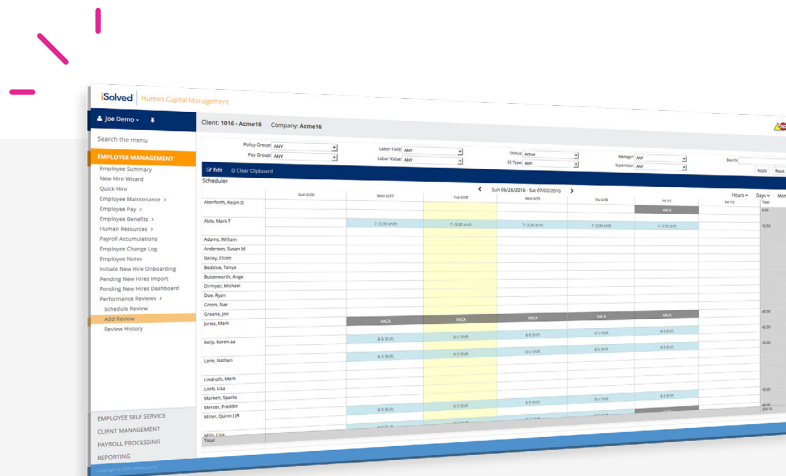
Scheduler
